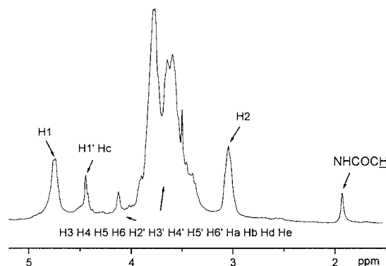
Figure 4 ^1\text{H-NMR} spectra of galactosylated chitosan.
